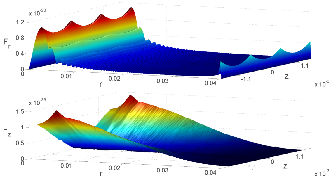
Figure 3.4. Radial self-force (top) and the absolute value of the axial self-force (bottom) of a single particle as a function of r and z near the midpoint of the trap using r^2 - z weighting factors. The oscillations are an artifact of interpolation/extrapolation, but persist regardless of which weighting factors are used. Also visible is how the force becomes more and more smooth as the cells shrink in size at larger radii.
