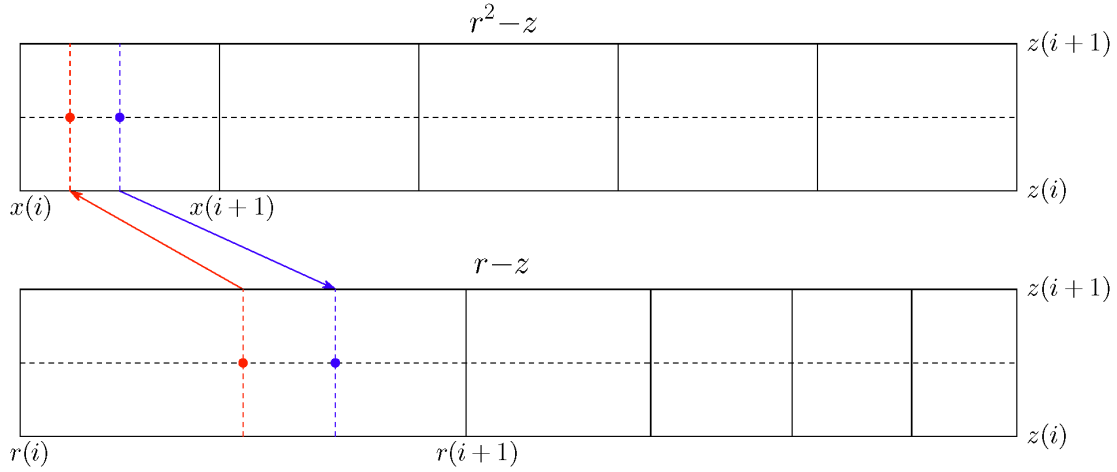
Figure 3.1. The two sets of coordinate grids (top: r^2 - z ; bottom: r - z ) show the difference between placing a particle at the center of a cell in r (shown in red) as opposed to placing it at the center in x or r^2 (shown in blue). Depending on which coordinate system is used, the surrounding grid points will be assigned different charge densities according to their relative proximity to the charge.
