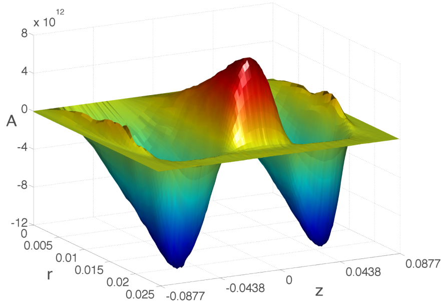
Figure 4.5. Mode shape for the first lower frequency with k_z = 3/2 (marked “B” in Figure 4.3).
