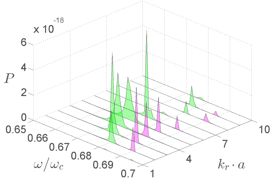
Figure 4.12. Waterfall plots of the RMS radial position FFT spectrum driven at 0.68\omega_c (green) and 0.7\omega_c (purple) for various radial wave numbers. In both cases, the peak frequencies undulate as k_r increases.
