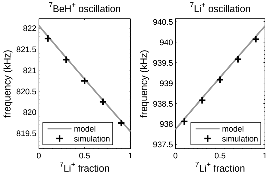
FIG. 4.10 Analysis of how the FTICR-MS spectral peaks for {}^7\text{BeH}^+ and {}^7\text{Li}^+ vary with fraction of {}^7\text{Li}^+ at a central density of 10^{12} \text{ m}^{-3} . It fits well with an analytical model using two charge columns in a grounded cylinder. The average percent error between the model and simulation is 0.006%.
