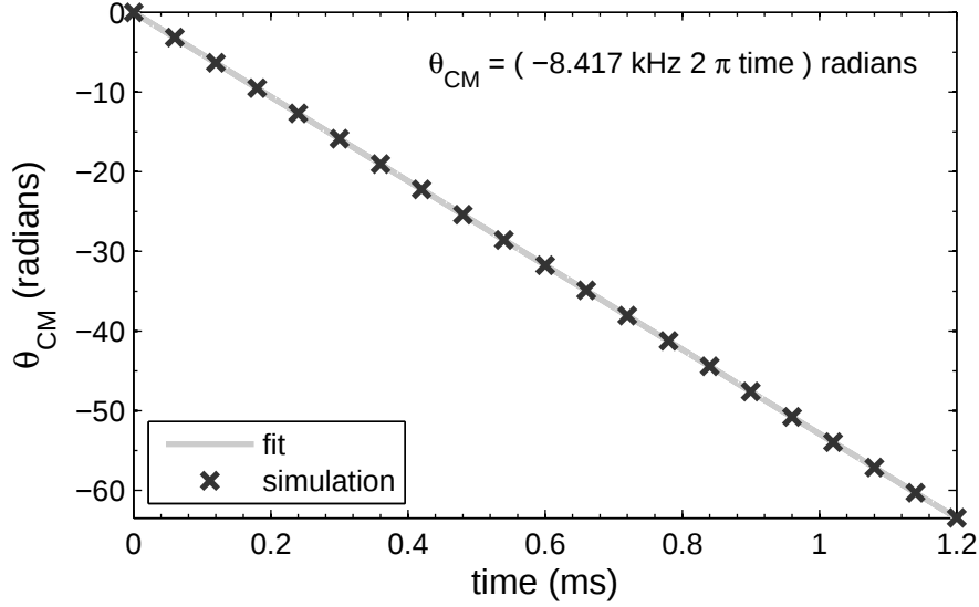
FIG. 3.11 This is a linear fit of the center-of-mass angle \theta_{cm} for a ^7\text{Be} ion plasma with a density of 10^{13} \text{ m}^{-3} and a 1 mm x-offset from the axis. The fitted diocotron frequency for an infinitely long plasma is 8.417 kHz. The fitted equation is written in the top right corner.
