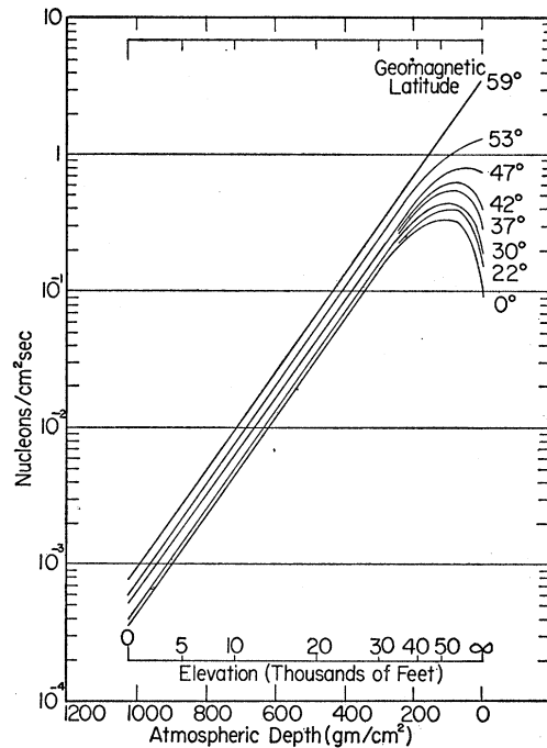
FIG. 4. Total nucleon flux vs atmospheric depth E_{\text{nucleon}} \geq 40 Mev.
