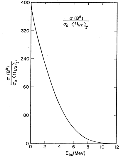
FIG. 2. The value of \sigma/\sigma_0\langle f\tau_{1/2} \rangle^2 versus excitation energy, E_{ex} , in \text{Ar}^{37} .
