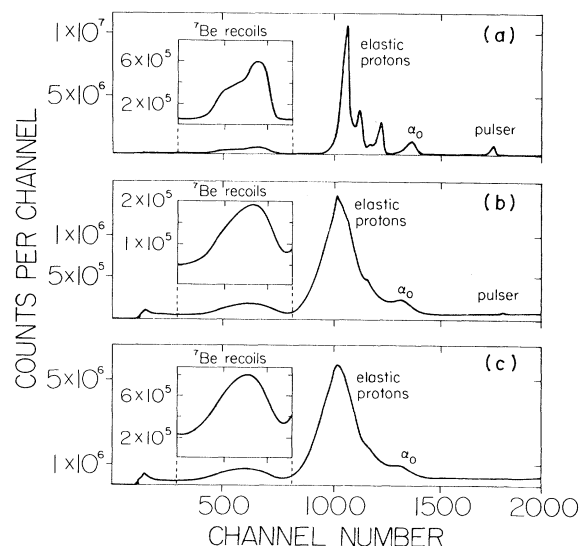
FIG. 2. Spectra for the {}^{10}\text{B}(p,\alpha){}^7\text{Be} reaction at 1.5\text{ MeV} from implanted detectors. (a) Detector implanted with 1.56 \times 10^8 {}^7\text{Be} nuclei at I_p \approx 1.3\text{ }\mu\text{A} . (b) Detector implanted with 1.6 \times 10^8 {}^7\text{Be} nuclei at I_p \approx 4.5\text{ }\mu\text{A} . (c) Detector in (b) with a total of 8 \times 10^8 {}^7\text{Be} nuclei implanted at I_p \approx 4.5\text{ }\mu\text{A} . Note that the quality of the spectrum is primarily a function of beam current, not the total integrated flux.
