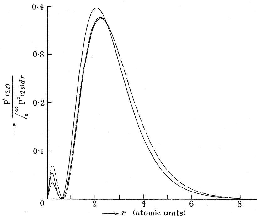
FIG. 2—Normalized P^2(2s) for Be. — from solution of Fock's equations, ( P_f^2 ). ---- from solution of equations of self-consistent field, ( P^2 ). - . - . - ditto, modified so that P(2s) is orthogonal to P(1s) , ( P_s^2 ).
