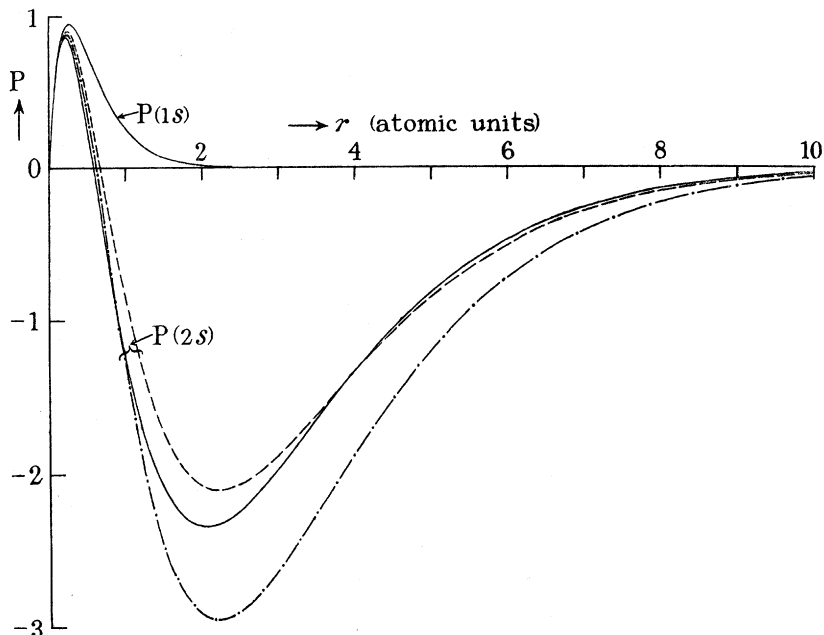
FIG. 1.—Unnormalized radial wave functions P(1s) , P(2s) , for Be. — from solutions of Fock's equations, ( P_f ). - - - - from solution of equations of self-consistent field, ( P_s ). - . - . - P(2s) from solution of equations of self-consistent field, modified so as to be orthogonal to P(1s) , ( P_s' ). (\frac{dP}{dr})_{r=0} = 10 in all cases. The difference between P_f(1s) and P_s(1s) is too small to be shown on the scale of the figure.
