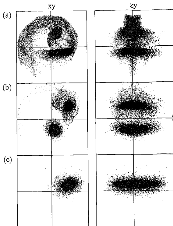
Figure 6. Snapshots in xy perspective (left) and zy perspective (right) at a late time during the detection period. (a) 50,000, (b) 150,000, and (c) 350,000 ions. The two masses have locked cyclotron modes in (c). The cubic trap boundary is indicated as the surrounding box.
