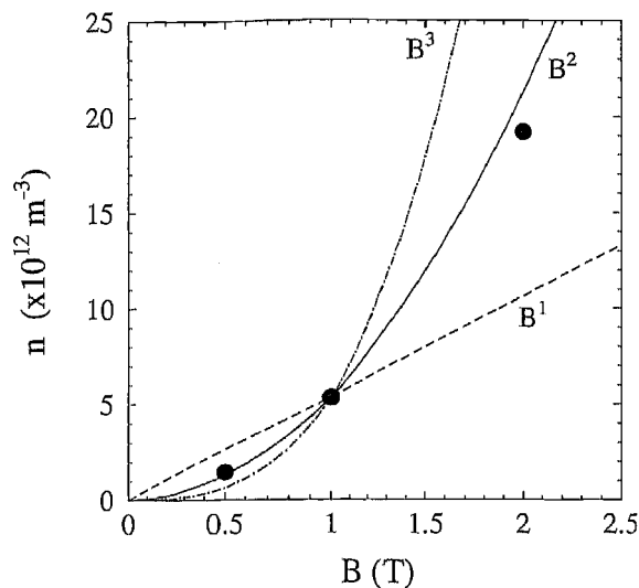
Figure 13. Magnetic field dependence of the minimum number density required to lock cyclotron modes. The solid circles are the simulation results at three different magnetic fields. The lines are three different assumed magnetic field dependencies, n proportional to B^1 , B^2 , and B^3 .
