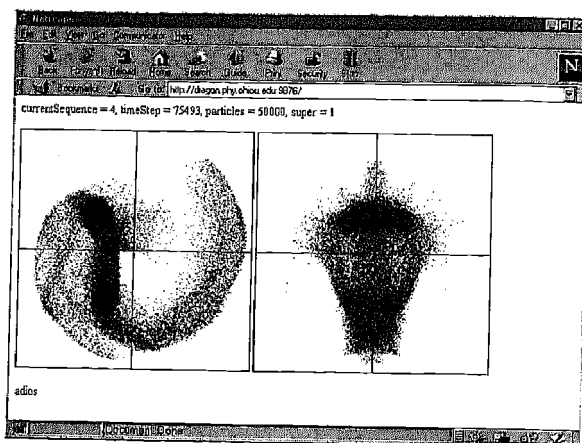
Figure 2. Real-time status of a simulation via an HTTP client. A popular web browser is used to query the PIC3D server on the status of an on-going simulation. The server responds by forking a new process that creates GIF images of the current time-step simulation, and sends this data back to the requesting web browser. The particle positions are plotted in xy (left) and yz (right) perspective.
