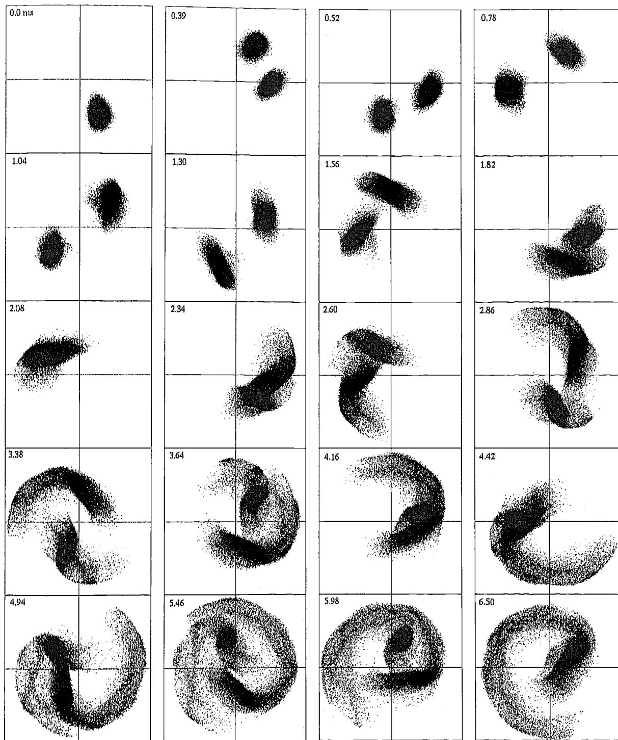
Figure 7. Snapshots of ion xy positions for the 50,000 ion simulation at selected times during the detection period. The cubic trap boundary is indicated.
