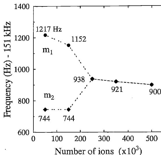
Figure 12. The frequency of coherent cyclotron motion, for the two species m_1 (100.0 u) and m_2 (100.3 u), as a function of the total number of confined ions. Results for five different simulations are shown with number of ions ranging from 50,000 to 500,000. Cyclotron phase locking occurs when the two masses have the same detected cyclotron frequency. The uncertainty is \pm 2 Hz. The lines are only meant to guide the eye. Other simulation parameters are listed in Table 1.
