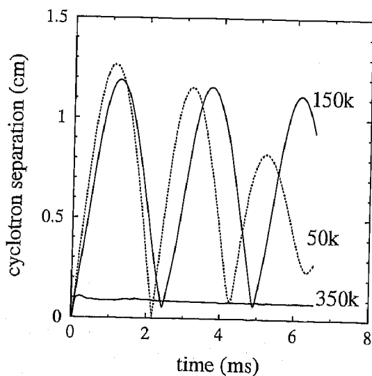
Figure 11. The separation distance between the centers of coherent cyclotron motion for the two masses for the 50,000, 150,000, and 350,000 ion simulations.
