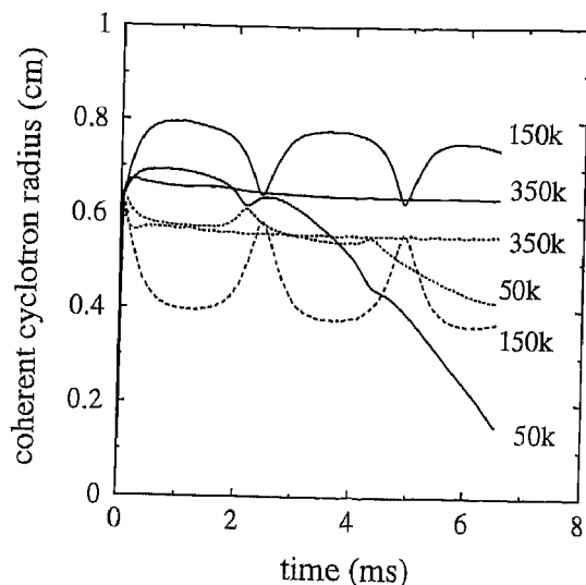
Figure 10. Evolution of the coherent cyclotron radii during the detection period for the two masses. (a) 50,000, (b) 150,000, and (c) 350,000 ion simulations. The 100.0 and 100.3 u mass species are plotted as solid and broken lines, respectively.
