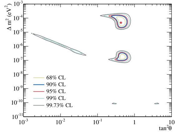
FIG. 4 (color). SNO-only neutrino oscillation contours, including pure \text{D}_2\text{O} day and night spectra, salt CC, NC, ES fluxes, with ^8\text{B} flux free and hep flux fixed. The best-fit point is \Delta m^2 = 4.7 \times 10^{-5} , \tan^2\theta = 0.43 , f_B = 1.03 , with \chi^2/\text{DOF} = 26.2/34 .
