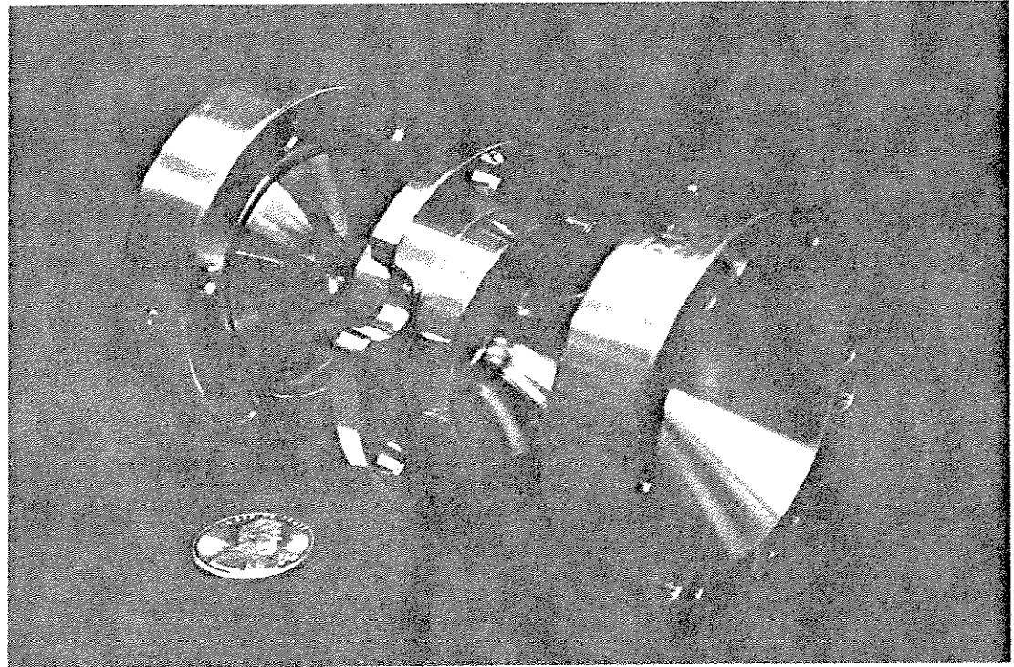
Figure 2. The three electrodes of the quadrupole ion trap shown in open array.
