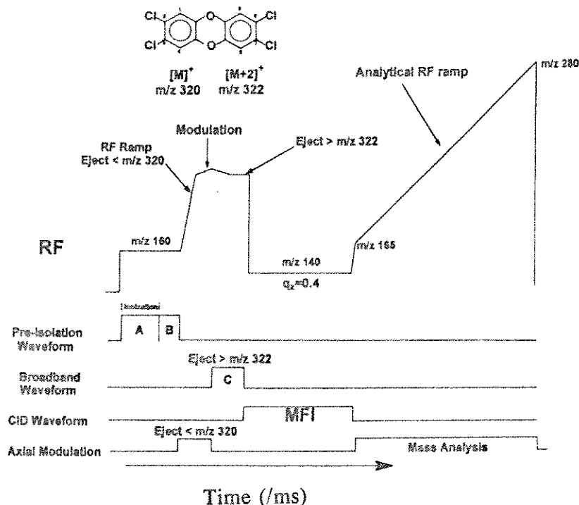
Figure 15. Scan function for MS/MS of dioxin ( T_4 CDD); the pre-scan for AGC is not shown.
