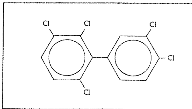
Congener 110
