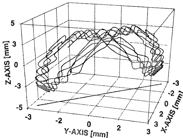
Figure 8. Trajectory of a trapped ion of m/z 105. The initial position was selected randomly from a population with an initial gaussian distribution (FWHM of 1 mm); q_x = 0.3 ; zero initial velocity. The projection on to the x - y plane illustrates planar motion in three-dimensional space. The trajectory develops a shape which resembles a flattened boomerang. Taken from Ref. 14.
