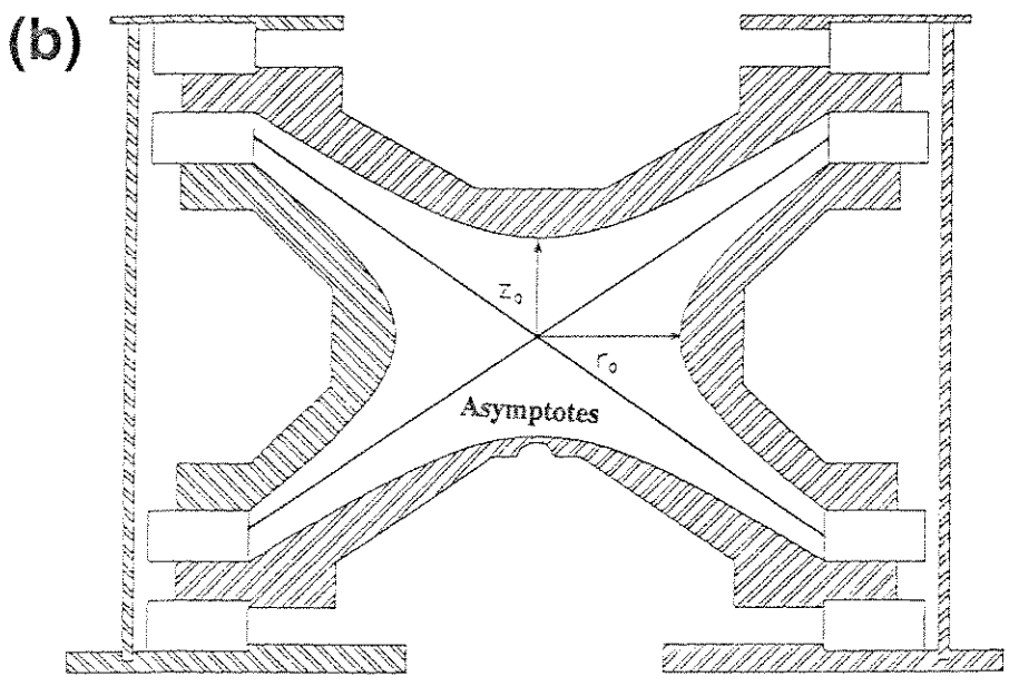
Figure 3. Quadrupole ion trap. (a) Photograph of an ion trap cut in half along the axis of cylindrical symmetry; (b) schematic diagram of the three-dimensional ideal ion trap showing the asymptotes and the dimensions r_0 and z_0 .
