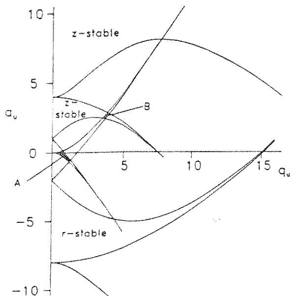
Figure 6. Mathieu stability diagram in (a_z, q_z) space for the quadrupole ion trap in both the r - and z -directions. Regions of simultaneous overlap are labelled A and B.
