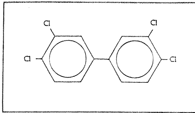
Congener 77
