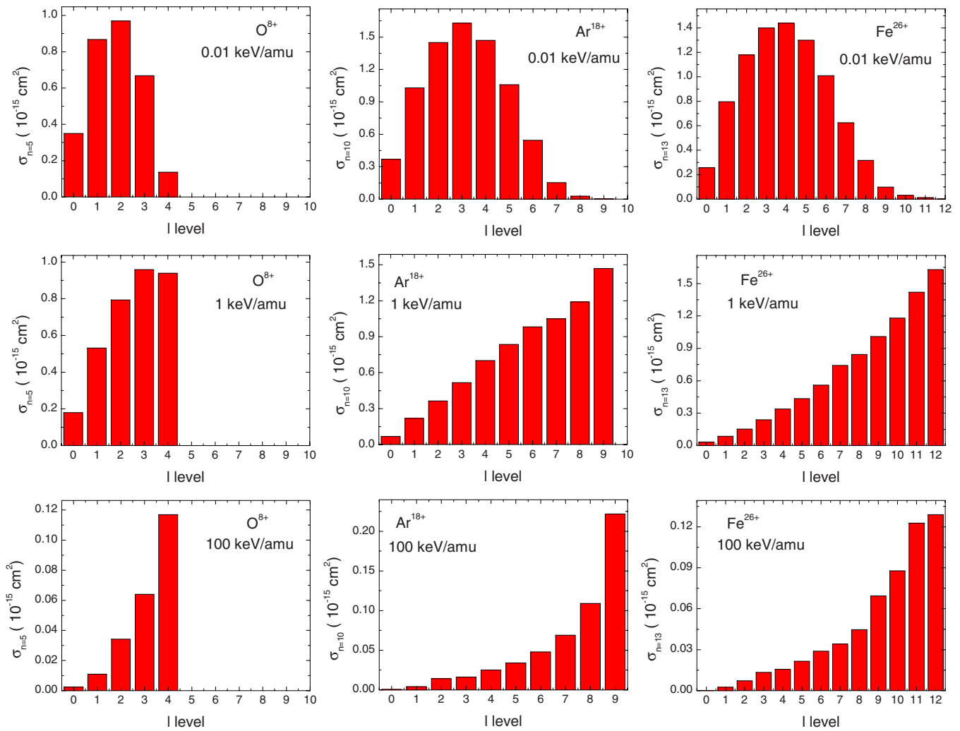
FIG. 5. (Color online) l -state selective single electron capture cross sections for 0.01, 1, and 100 keV/amu O^{8+} , Ar^{18+} , and Fe^{26+} ions impinging on H_2O .
